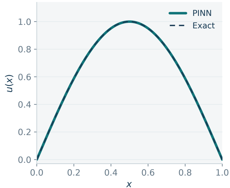
A A learned solution
